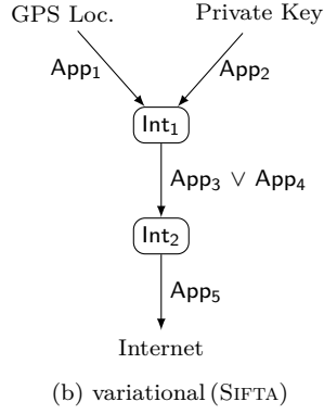
Fig. 3: Example of an inter-app data flow, non-variational and variational. Edges are annotated with app names instead of component names.
