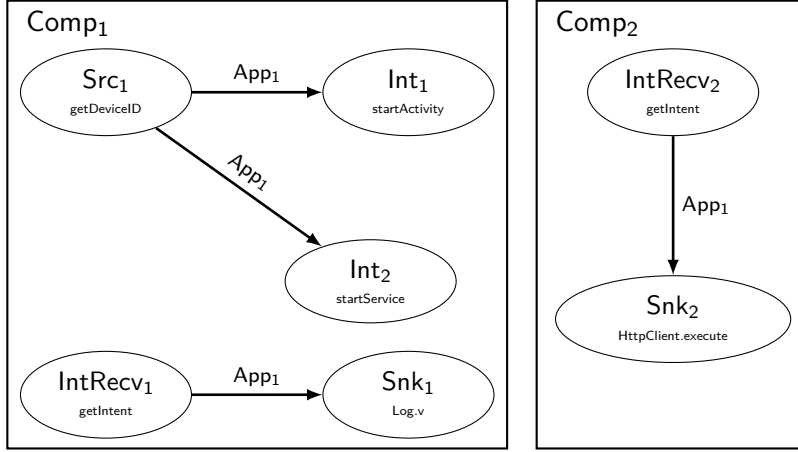
Fig. 4: An app with two components ( \text{Comp}_1, \text{Comp}_2 \in \text{Comp} ) with intra-component flows, connecting a source ( \text{Src}_1 \in \text{PrivSrc} ) with two intent calls ( \text{Int}_1, \text{Int}_2 \in \text{PubSnk} ) as well as two intent receivers ( \text{IntRecv}_1, \text{IntRecv}_2 \in \text{PrivSrc} ) with two sinks each ( \text{Snk}_1, \text{Snk}_2 \in \text{PubSnk} ). The apps involved are annotated to the edges.
