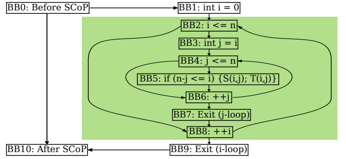
Fig. 3: Schematic view of the control-flow graph of Figure 1. The highlighted region marks the SCoP detected by POLLY.
