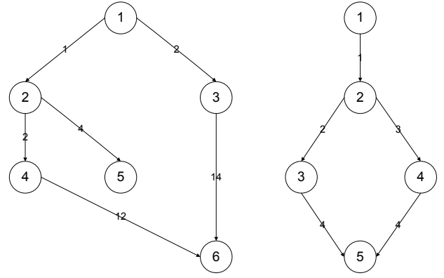
Figure 9: Resulting graph structures.
